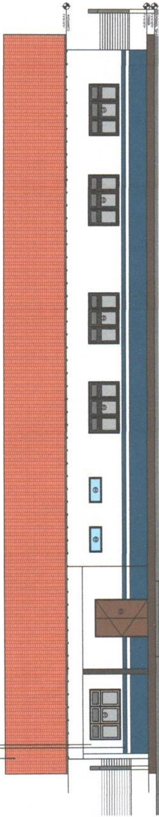
1 - FACHADA PRINCIPAL ESCALA 1/100
