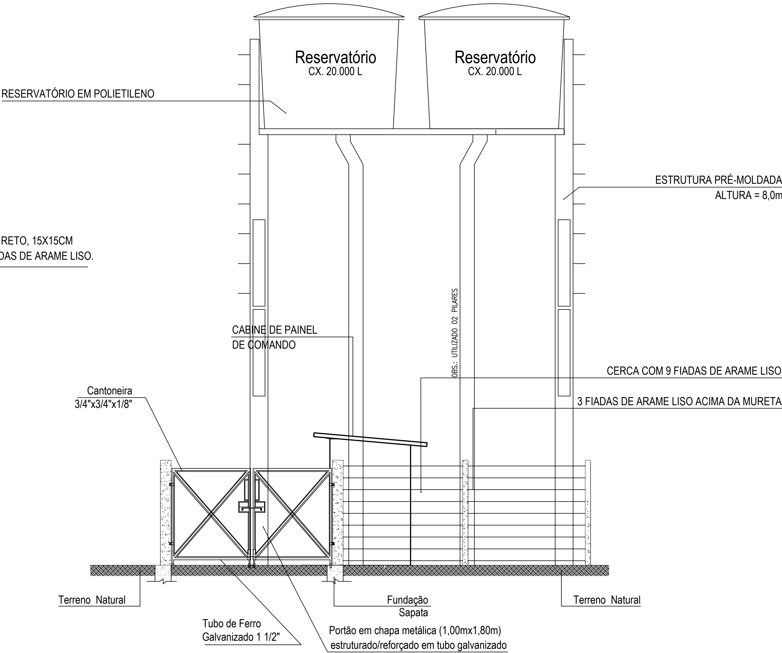
VISTA FRONTAL
